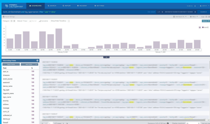
Log search
